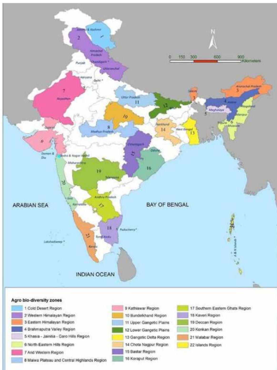
Fig 3.20. Agrobiodiversity Hotspots in India
