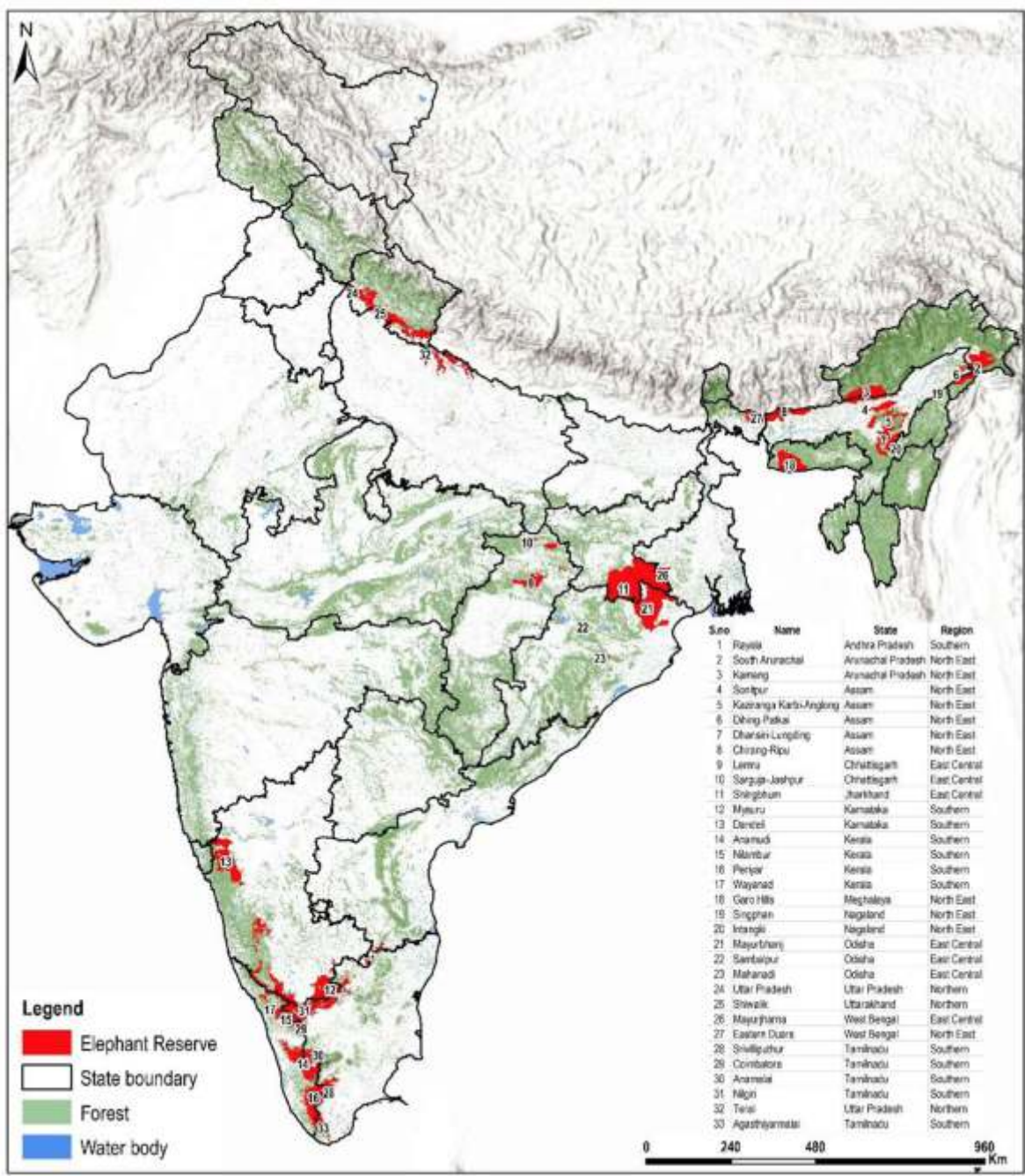
Fig 3.15. Elephant Reserves of India
