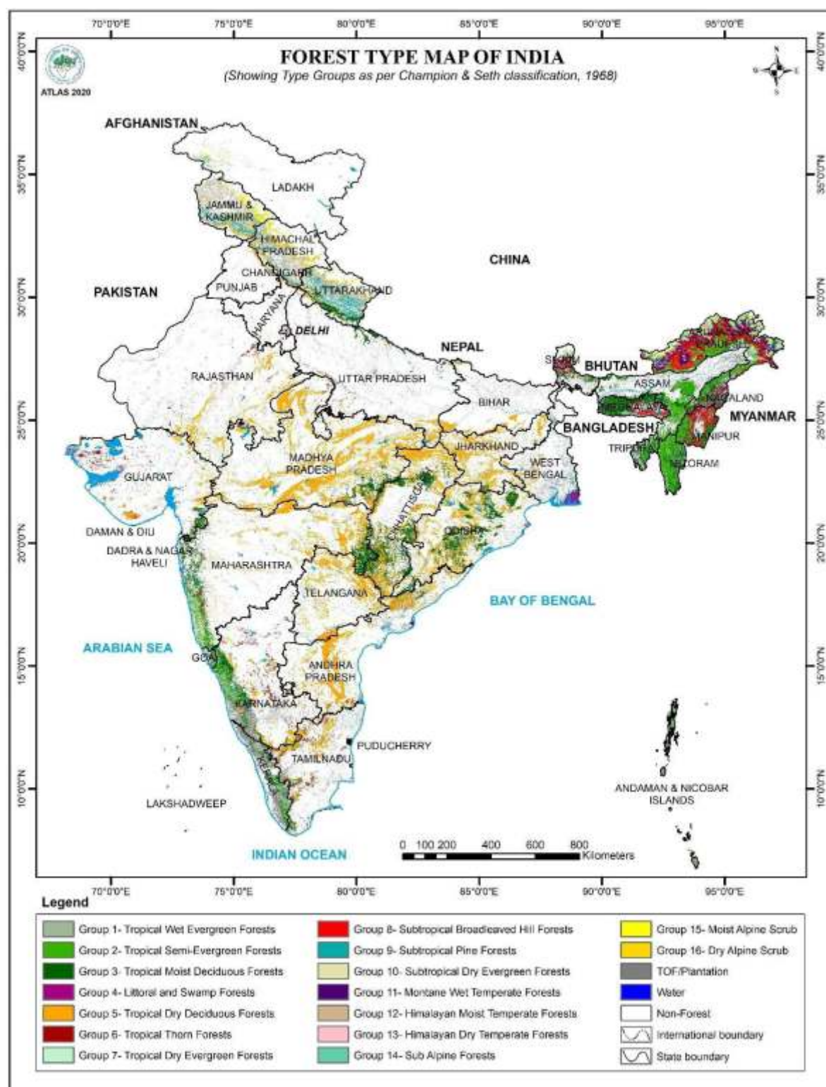
Fig 3.2. Distribution of Forest Types and TOF/ Plantation in India
