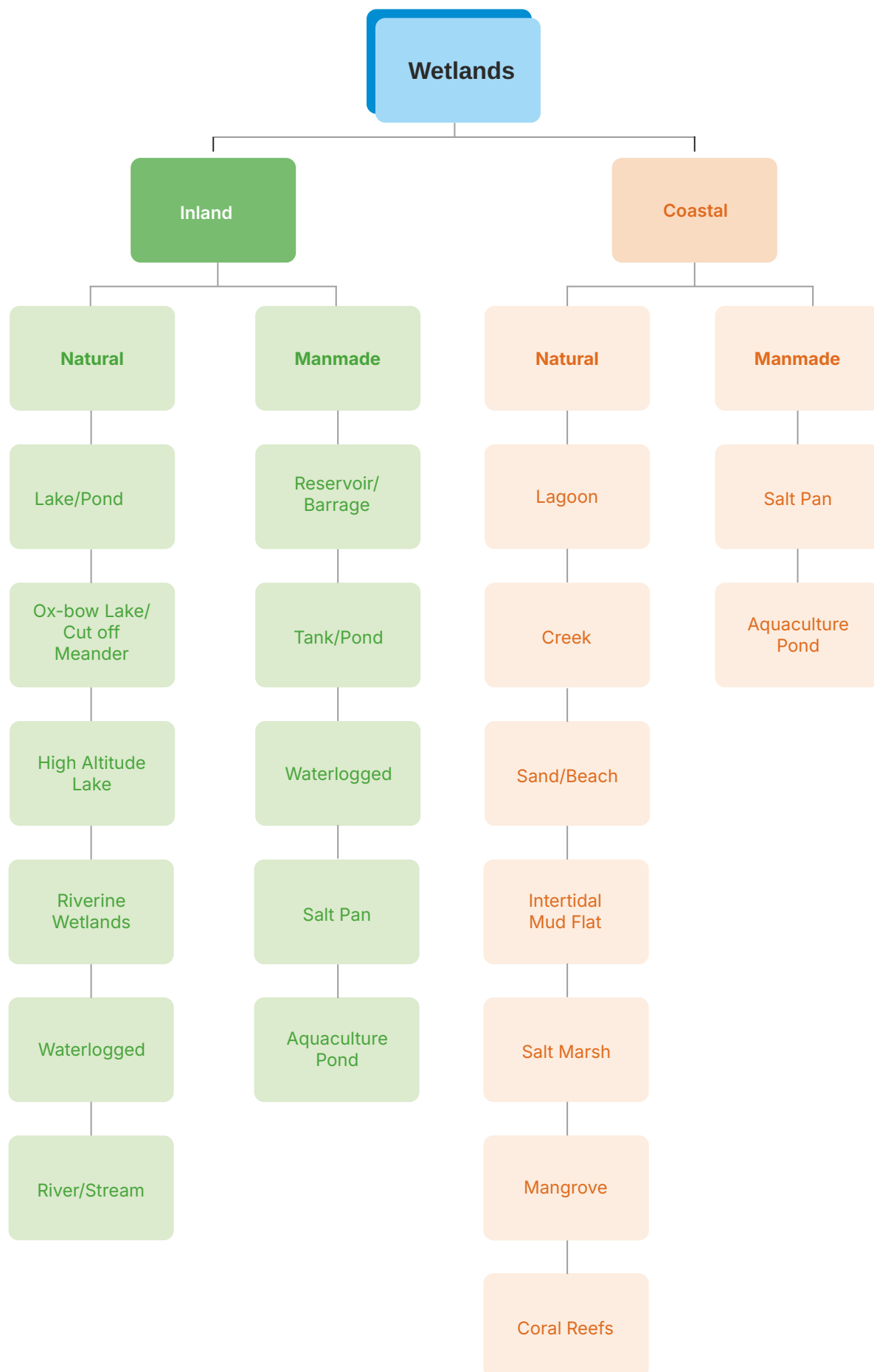
Fig 3.18. Three-Level Classification of Wetlands Adopted for the Preparation of National Atlas of Wetlands
