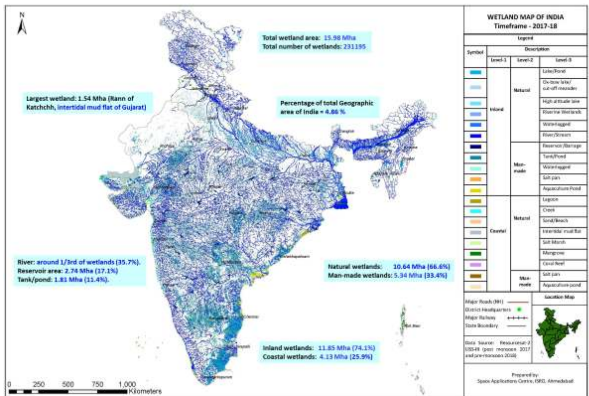
Fig 3.6. Wetland map of India
