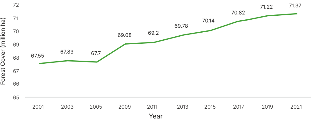
Fig 3.3. Changes in Forest Cover (2001-2021)
