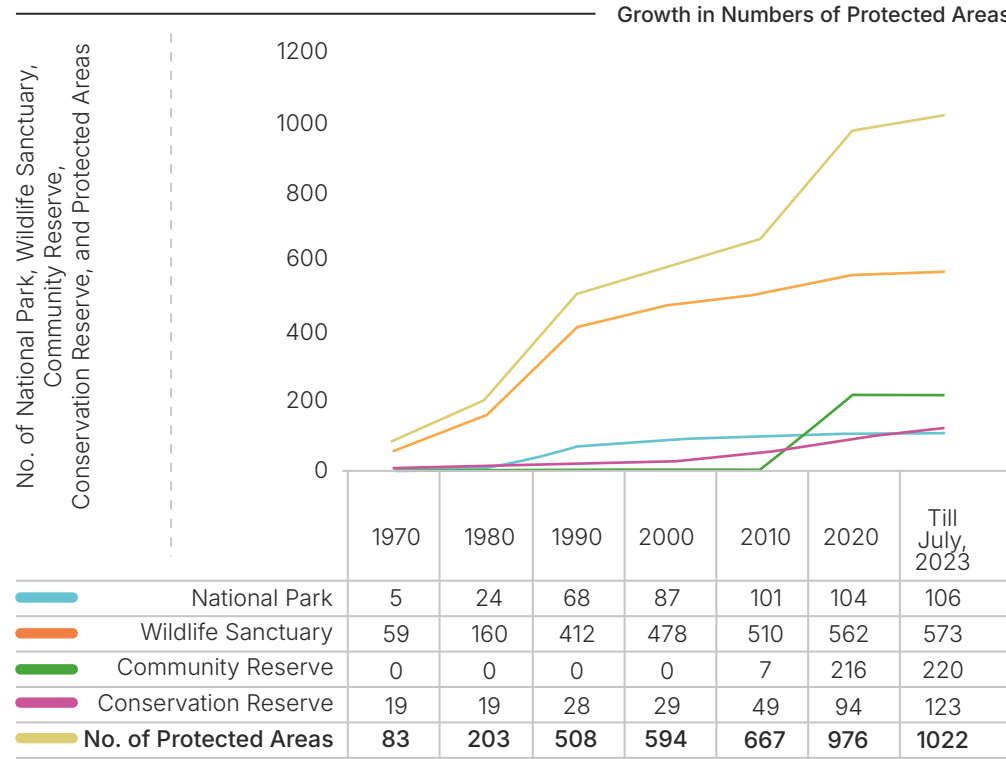
Fig 3.13. Growth in number of Protected Areas during 1970 - July, 2023
