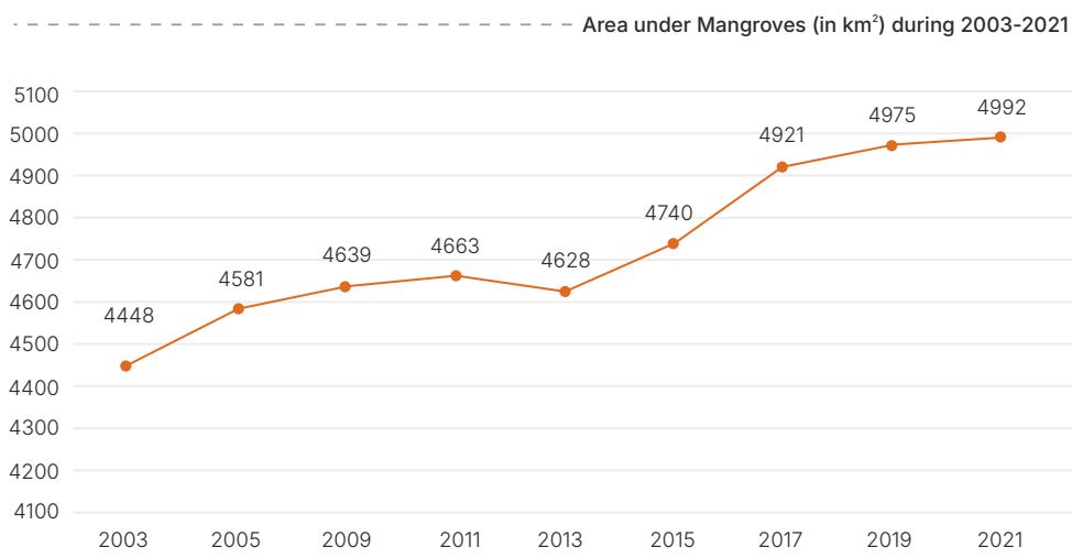
Fig 3.8. Mangrove Cover in India
